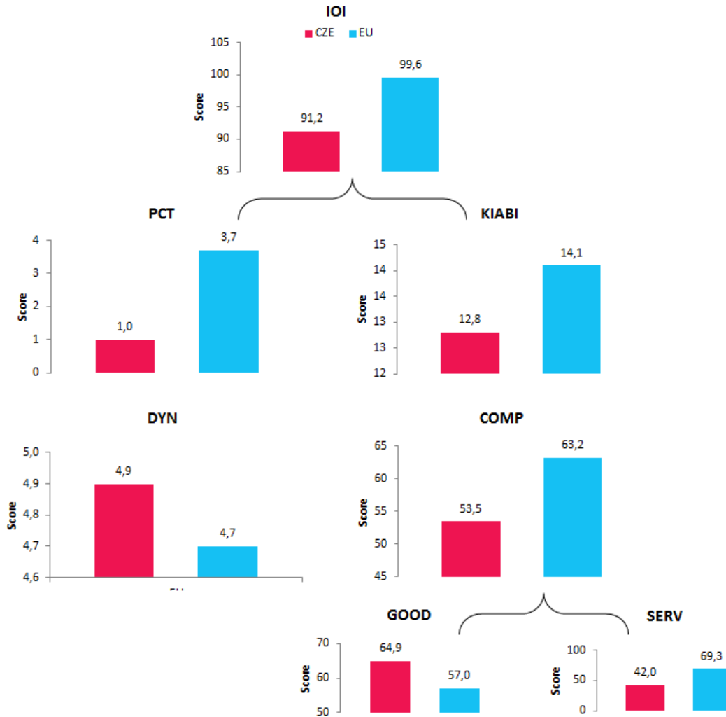
Fig. 1.5: IOI 2017 CR and EU
